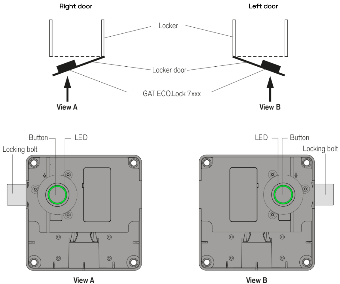
Figure 3.1 – Locker door hinge definition (left / right)
