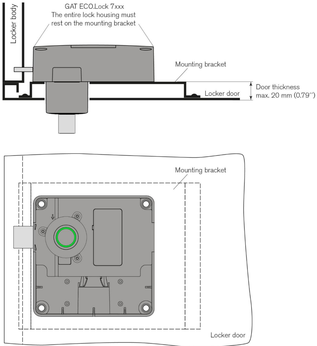
Figure 3.10 - Installation of the GAT ECO.Lock on a single-wall metallic door
