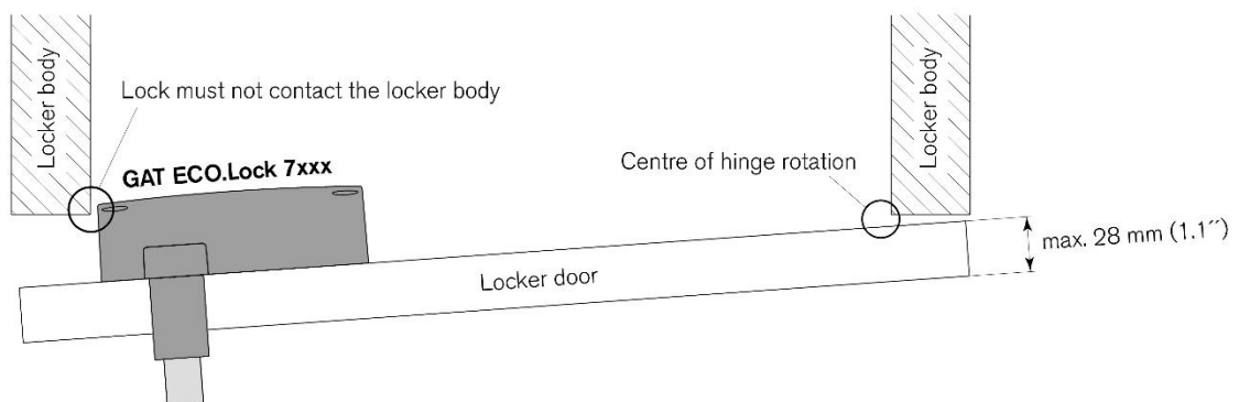
Figure 3.2 – Width and thickness of the locker door
