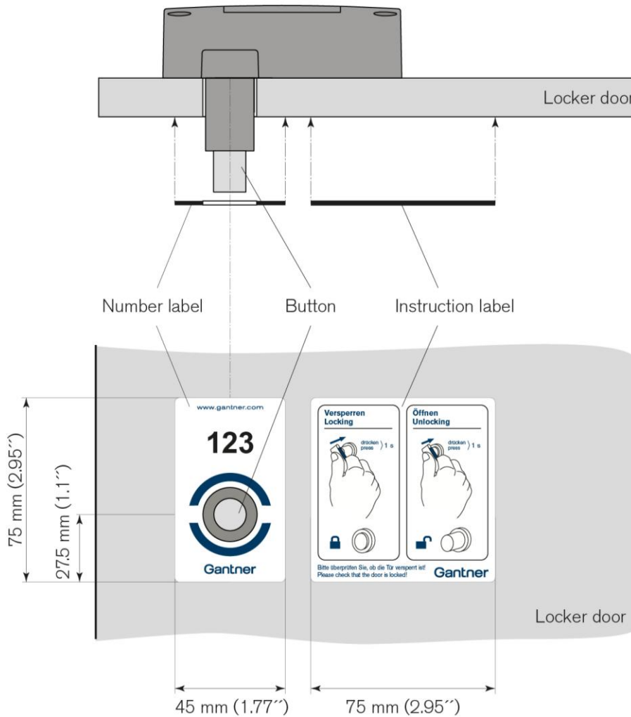
Figure 3.12 – Label attachments for right-hinged door
