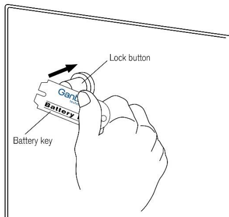
Figure 4.3 – Activating the GAT ECO.Lock with the RFID battery cover key
