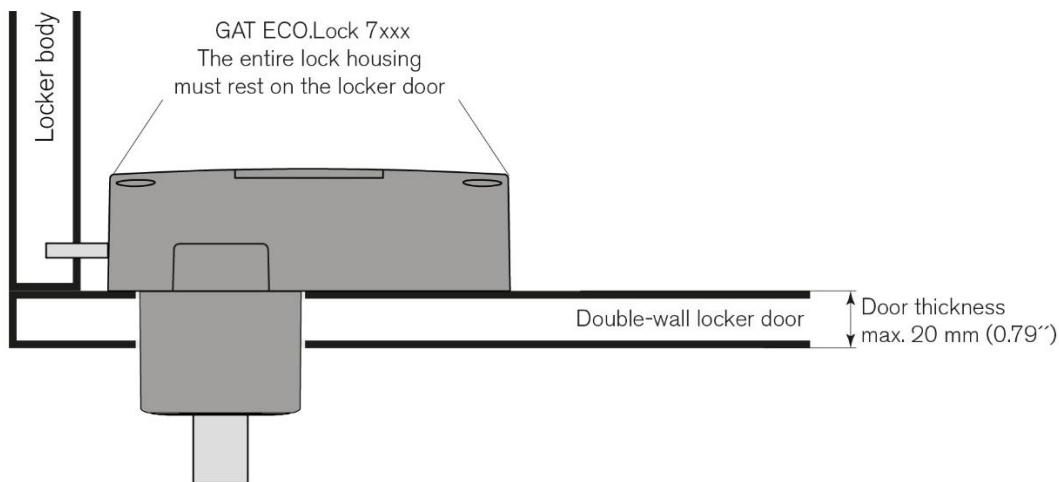
Figure 3.11 – Installation of the GAT ECO.Lock on a double-wall metallic door
