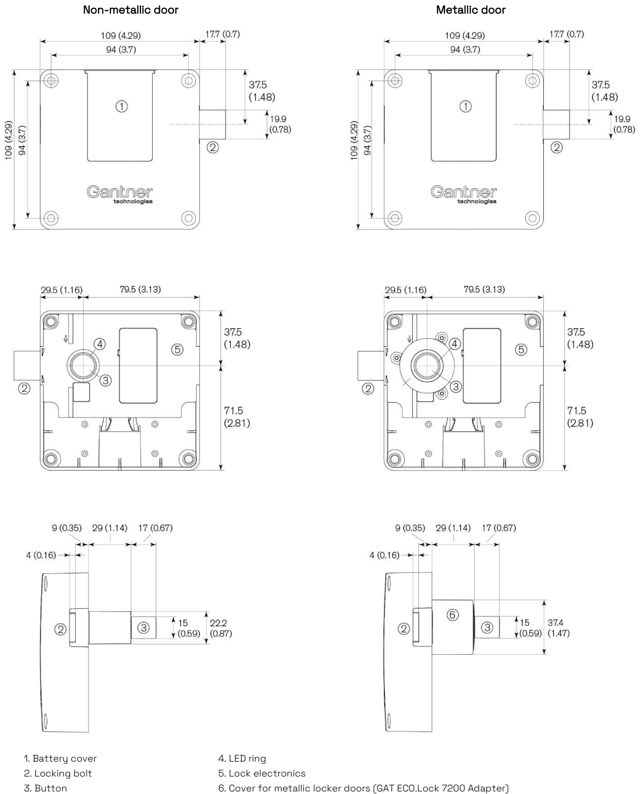
Figure 3.3 – GAT ECO.Lock dimensions and components
