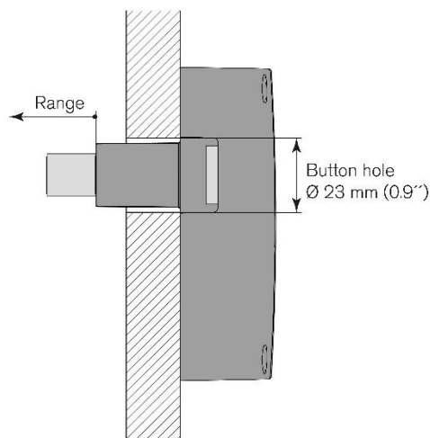
Figure 3.4 – Diameter of the button drill hole for non-metallic doors
